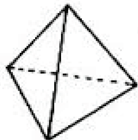
tetrahedron
