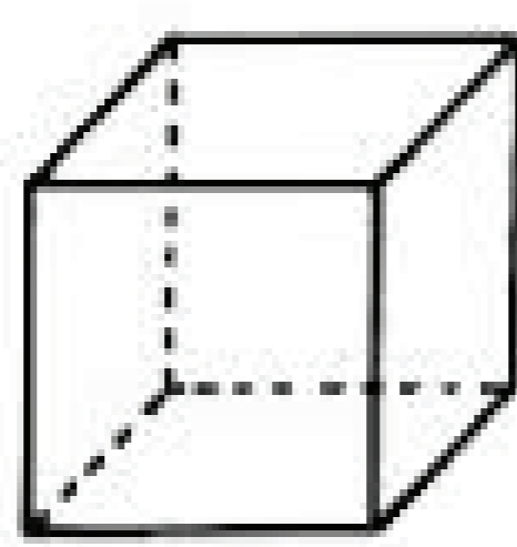
hexahedron
