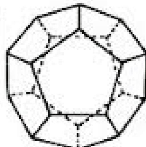
dodecahedron
