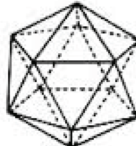
icosahedron
