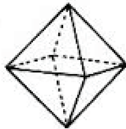
octahedron
