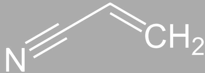
acrylonitrile
